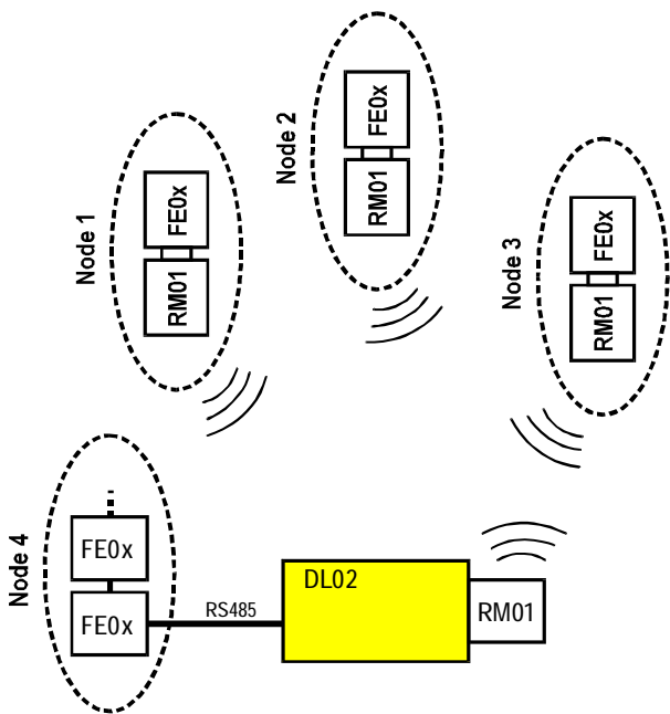
Example of a wireless network composed by 4 measurement nodes
